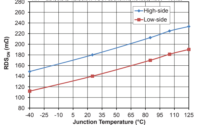
RDS ON vs. Temperature
